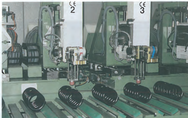
Signierlinie Colour code marking plant
