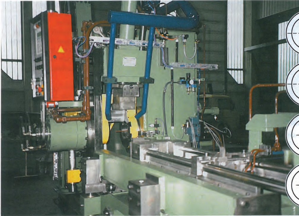
Hydraulische Augenrollmaschine Hydraulic Eye-Rolling Machine
